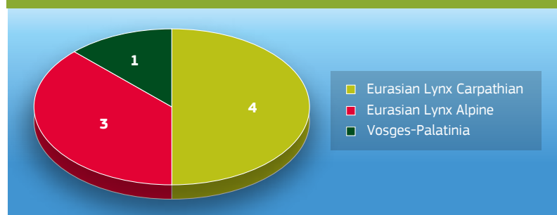
Figure 4. Number of LIFE projects targeting Eurasian lynx by population (1992-2011)
