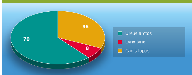
Figure 1. Number of LIFE projects targeting LC species (1992-2011)
