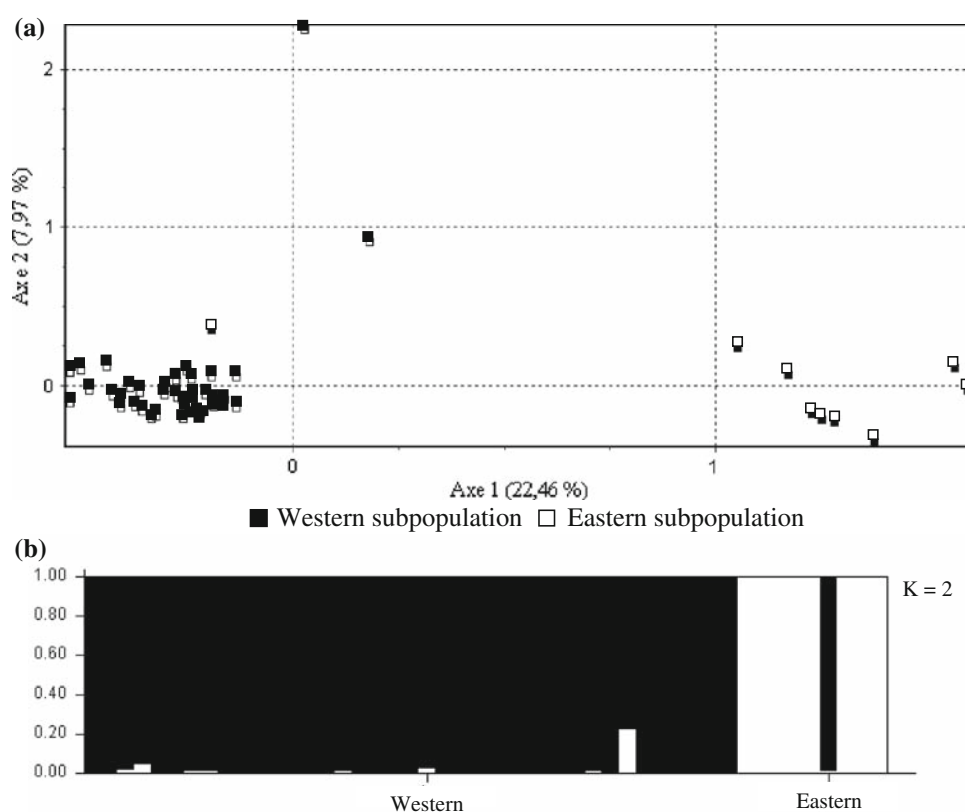
Fig. 4 (a) Distribution of individuals according to genotype based on factorial correspondence analysis (FCA), and (b) Graphical representation of the STRUCTURE programme. In both cases individuals belonging to the eastern and western populations are indicated in white and black, respectively
