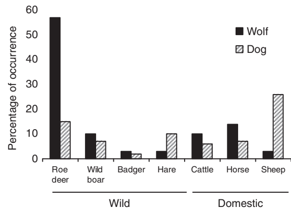
Figure 2 The per cent occurrence of wild and domestic prey in the feces of wolves Canis lupus ( n=31 ) and dogs Canis familiaris ( n=39 ) collected in the Basque Country, Spain, in 2003 and 2004.
