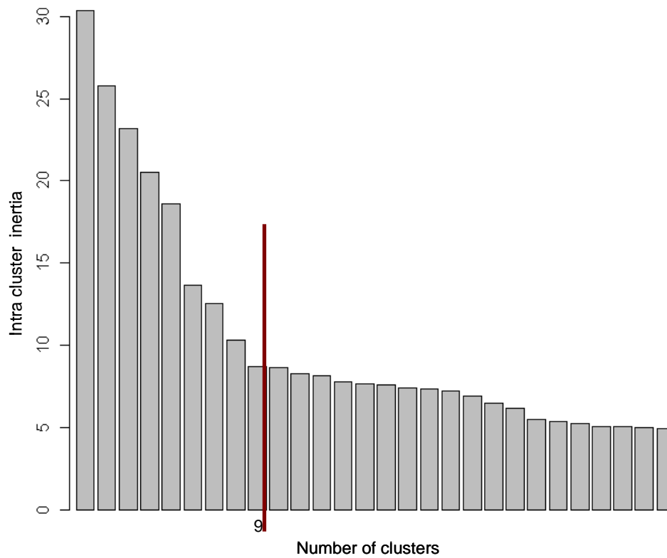
Figure 1: Bar chart of the sum of intra-cluster inertias for different numbers of clusters. The red line indicates the point of the changing slope.
